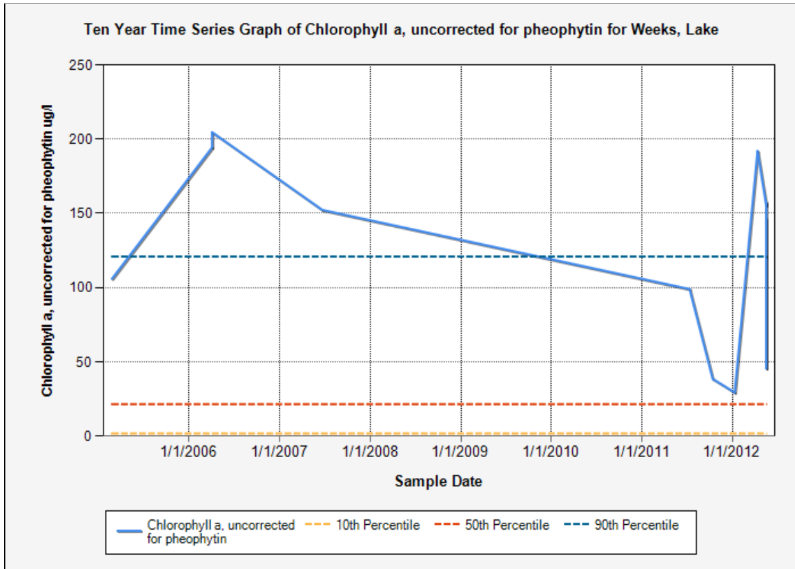
Figure 8. Recent Chlorophyll a graph for Lake Weeks vii
