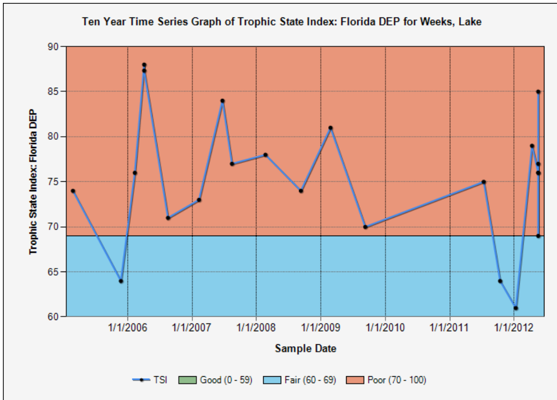
Figure 7. Recent Trophic State Index (TSI) graph for Lake Weeks vi
