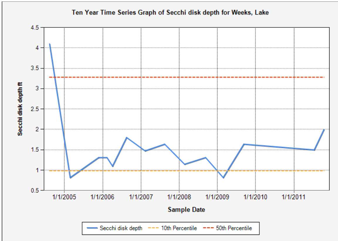
Figure 9. Recent Secchi Disk graph for Lake Weeks viii
